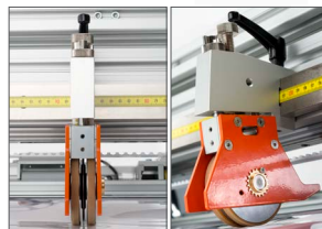
Slimline lengthwise rotary crush cutter, single or twin, (optional)
